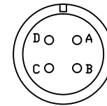
MS3102A22-22P Motor Cable Connector 접속도
