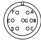
MS3102A24-10P Motor Cable Connector 접속도
