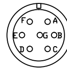
MS3102A24-10P Motor Cable Connector 접속도
